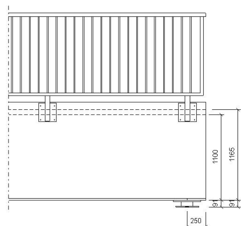
Detail Lager
